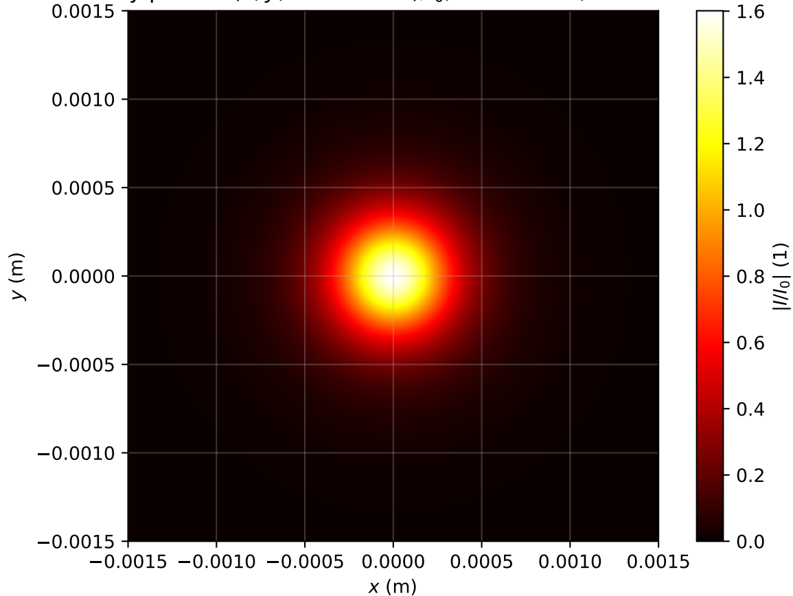
Intensity profile I(x, y, z = 1.672m)/I_0 , Pin=0.9Pcr, artificial time
